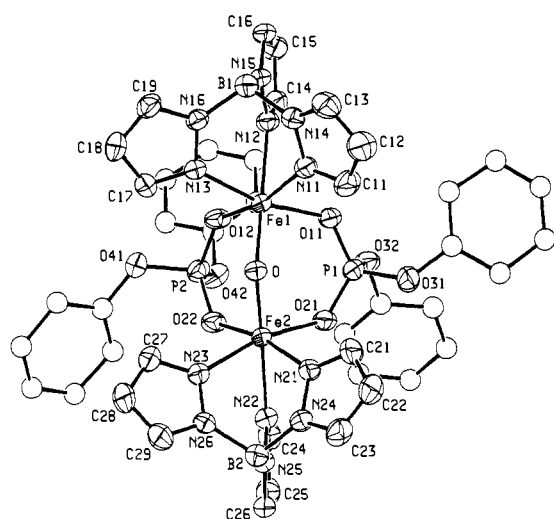
Figure 2. Structure of ( \mu -oxo)bis( \mu -diphenylphosphato)bis(hydrotris(1-pyrazolyl)borato)diiron(III) ( 3 ) showing the 40% probability thermal ellipsoids and atom-labeling scheme. The phenyl ring carbon atoms are depicted as spheres with an arbitrary B value of 3.0 \text{ \AA}^2 . For clarity, hydrogen atoms are omitted and the phenyl ring carbon atoms are not labeled. Selected interatomic distances ( \text{\AA} ) and angles ( ^\circ ) are as follows: Fe1-O 1.812 (5), Fe2-O 1.804 (5), Fe1-O11 2.059 (5), Fe1-O12 2.041 (5), Fe2-O21 2.045 (5), Fe2-O22 2.035 (5), Fe1-N11 2.137 (7), Fe1-N13 2.121 (6), Fe1-N12 2.213 (6), Fe2-N21 2.121 (6), Fe2-N23 2.142 (6), Fe2-N22 2.210 (7), Fe1...Fe2 3.337 (1), Fe1...P1 3.217 (2), Fe1...P2 3.210 (2), Fe2...P1 3.213 (2), Fe2...P2 3.205 (2), O11...O21 2.566 (7), O12...O22 2.576 (7), Fe1-O-Fe2 134.7 (3), O-Fe1-N12 179.8 (3), O-Fe2-N22 178.6 (2), N-Fe-N 81.0 (2)-85.3 (2).
